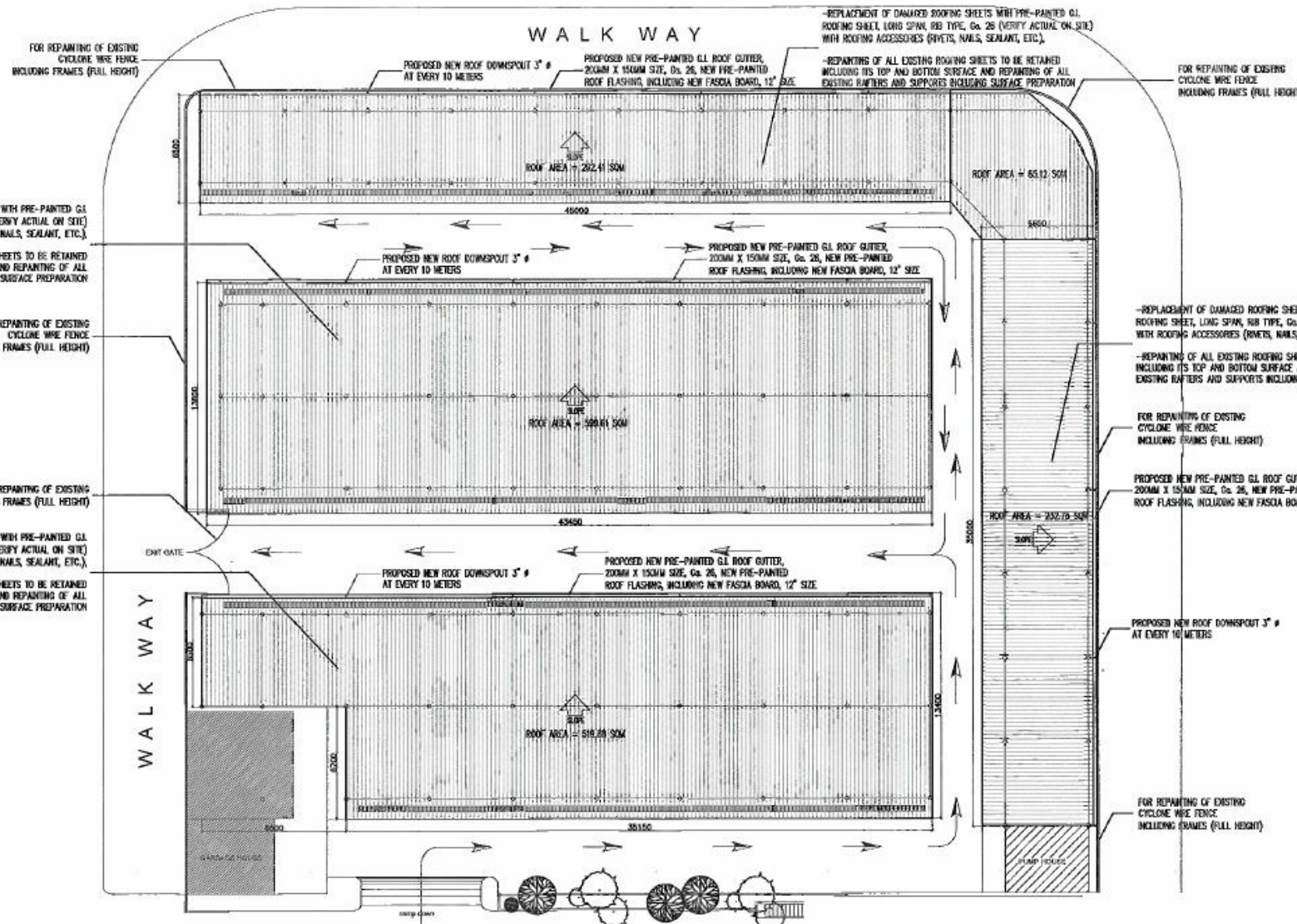
1 PROPOSED ROOFING PLAN A-02 SCALE 1:275 M.
