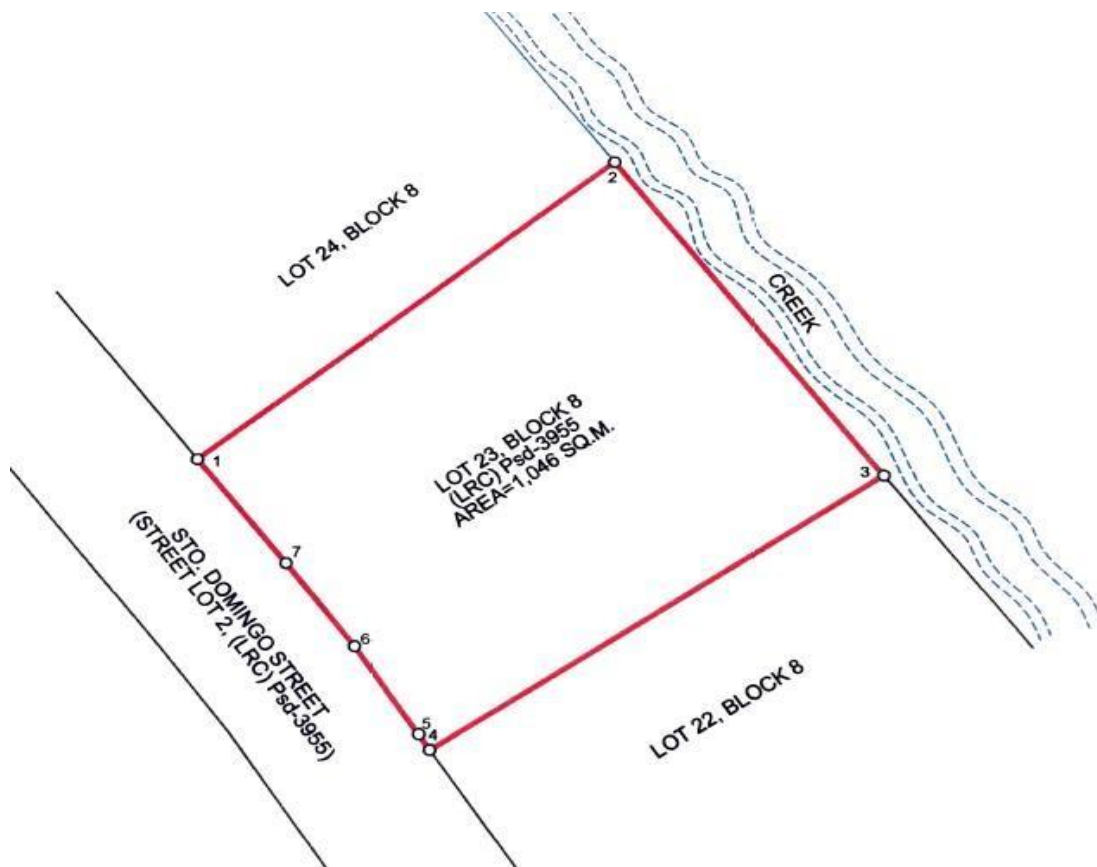
LOT PLAN
