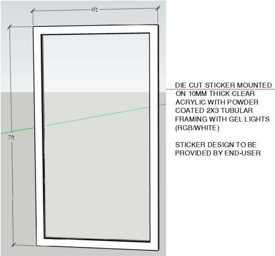
MAGAZINE PHOTO FRAME PROPOSED DETAIL 1 A-03 SCALE NTS
